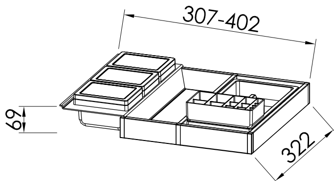
ORGANIZATOR PREDALA ZG. 350 - PRI OUN 120 DRAWER ORGANIZER UPPER 350 - FOR OUN 120
